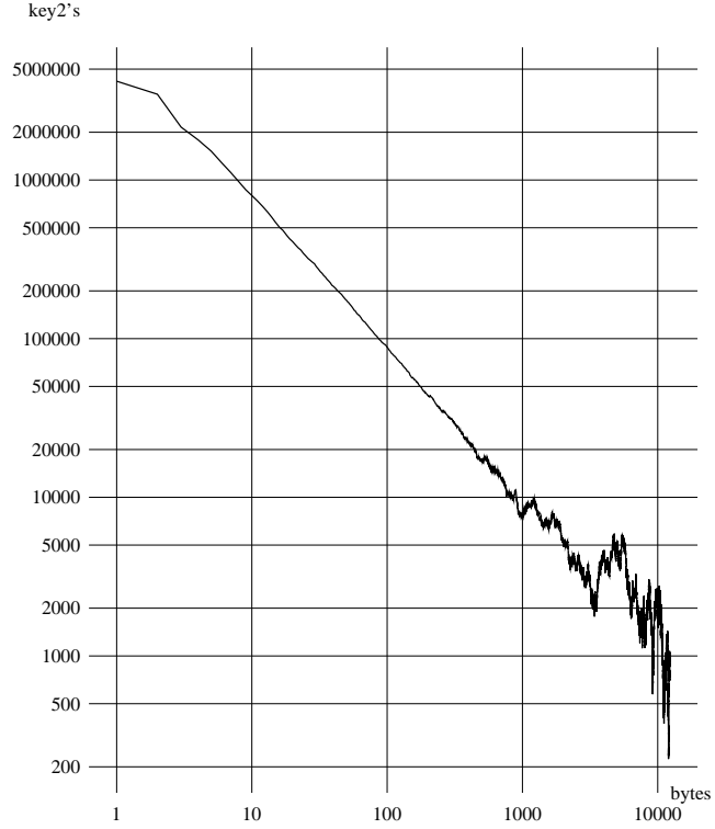
Fig. 1. Decrease in the number of key2 candidates using varying amounts of known plaintext. These results are for the PKZIP contest file and are fairly typical, though the entry 12000 is unusually low. (logarithmic scaling).
